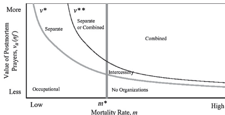
Fig. 3. Equilibrium conditions for three types of cooperation.
