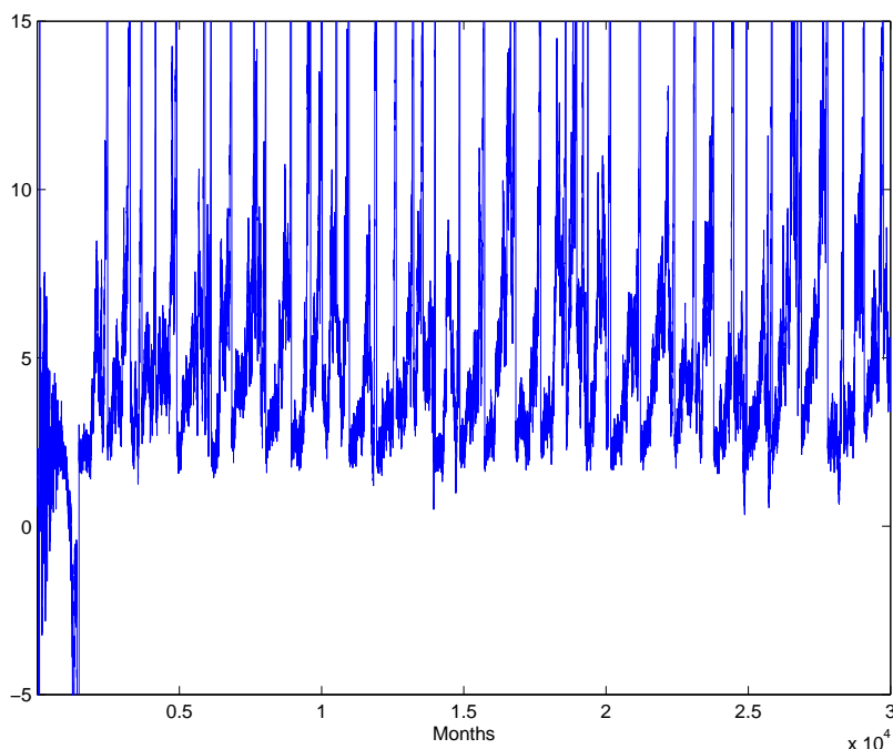
FIGURE 17. Long-run inflation dynamics with \theta_0 = -1.0 , using the end-of-sample estimate as the initial condition.
