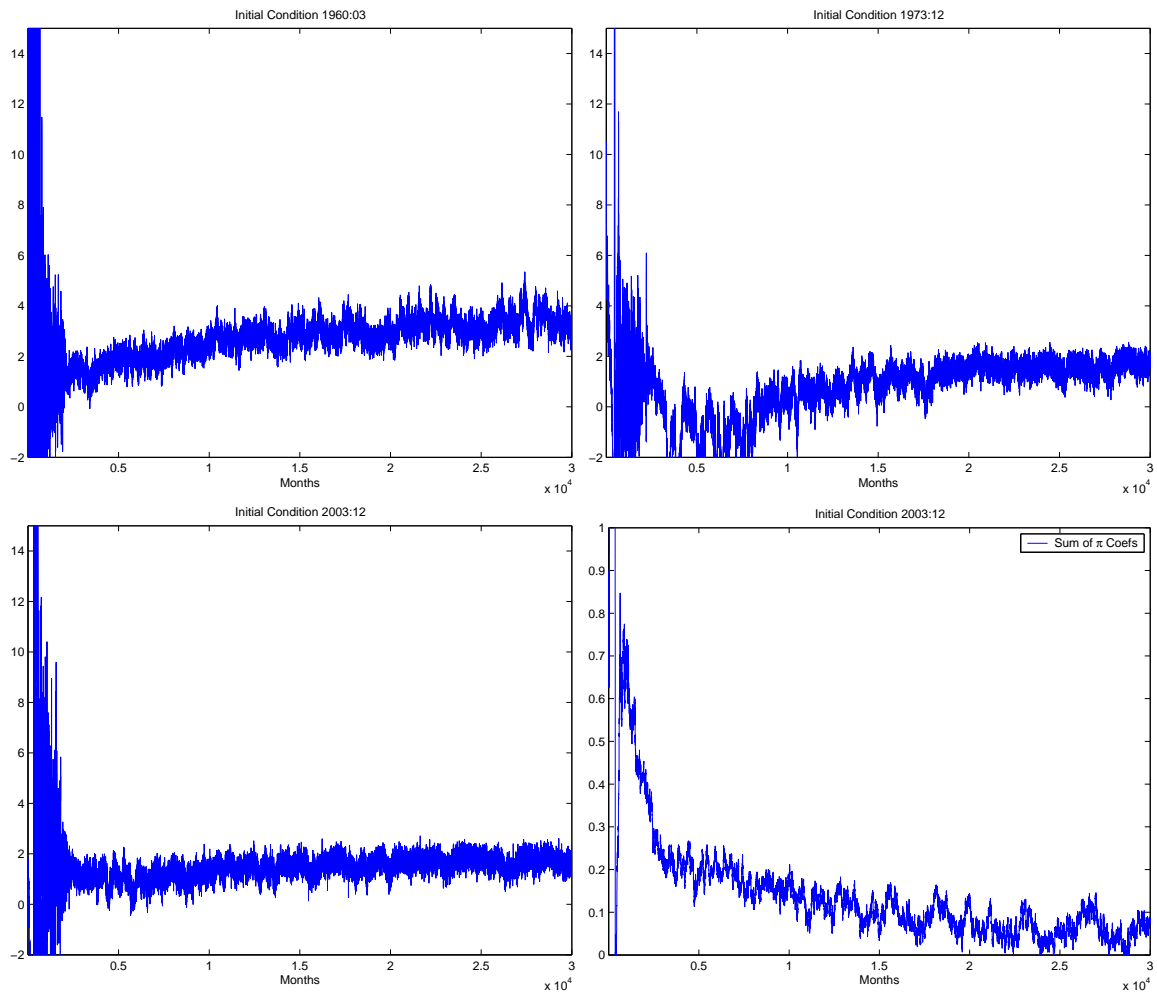
FIGURE 18. Government's inflation choice in long Monte Carlo simulations, using the different estimated initial conditions.
