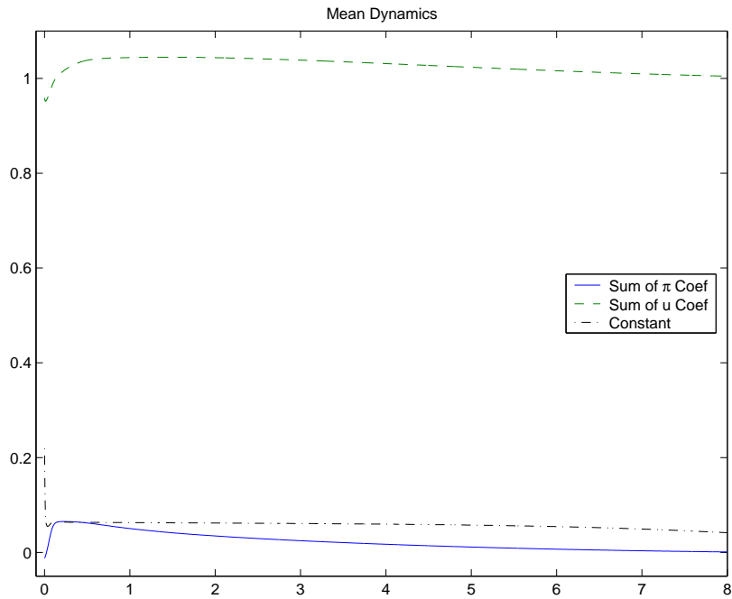
FIGURE 16. Mean dynamics for the baseline estimates, initialized at the start of the sample.
