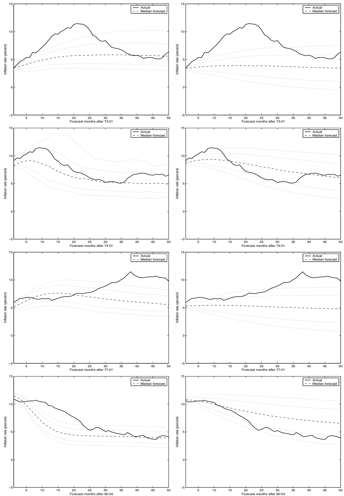
FIGURE 13. Dynamic forecasts of inflation with 68% and 90% error bands from our learning model (left column of graphs) and from BVAR(13) (right column of graphs), using as initial estimated conditions at 73:01, 74:01, 77:01, and 80:04.
