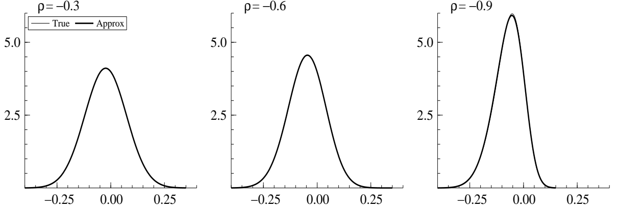
Figure 4: The marginal density of \eta_t given d_t = 1 for \rho = -0.3, -0.6, -0.9 (left, middle, right). The value of \sigma is set to 1 in this example.
