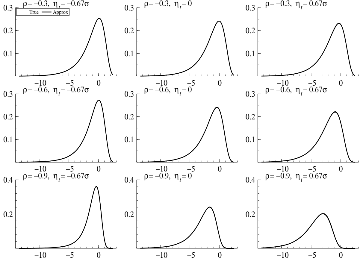
Figure 3: The conditional density of \xi_t given d_t = 1 and \eta_t = -0.67\sigma, 0, 0.67\sigma (left, middle, right) for \rho = -0.3, -0.6, -0.9 (top, middle, bottom). The value of \sigma is set to 1 in this example.
