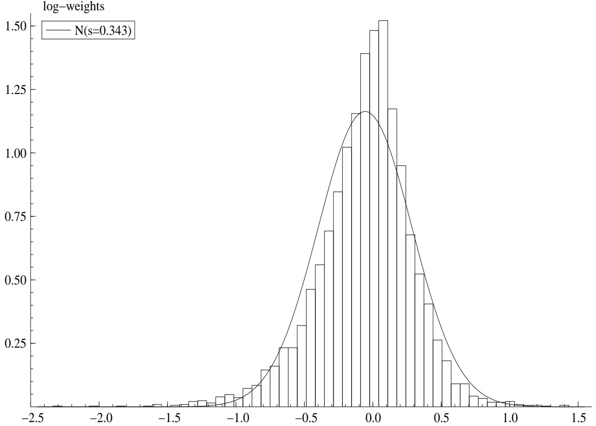
Figure 10: Sampling result of log-weights \log(w^{(i)} \times M) for the TOPIX series. Shows histogram and fitted normal density.
