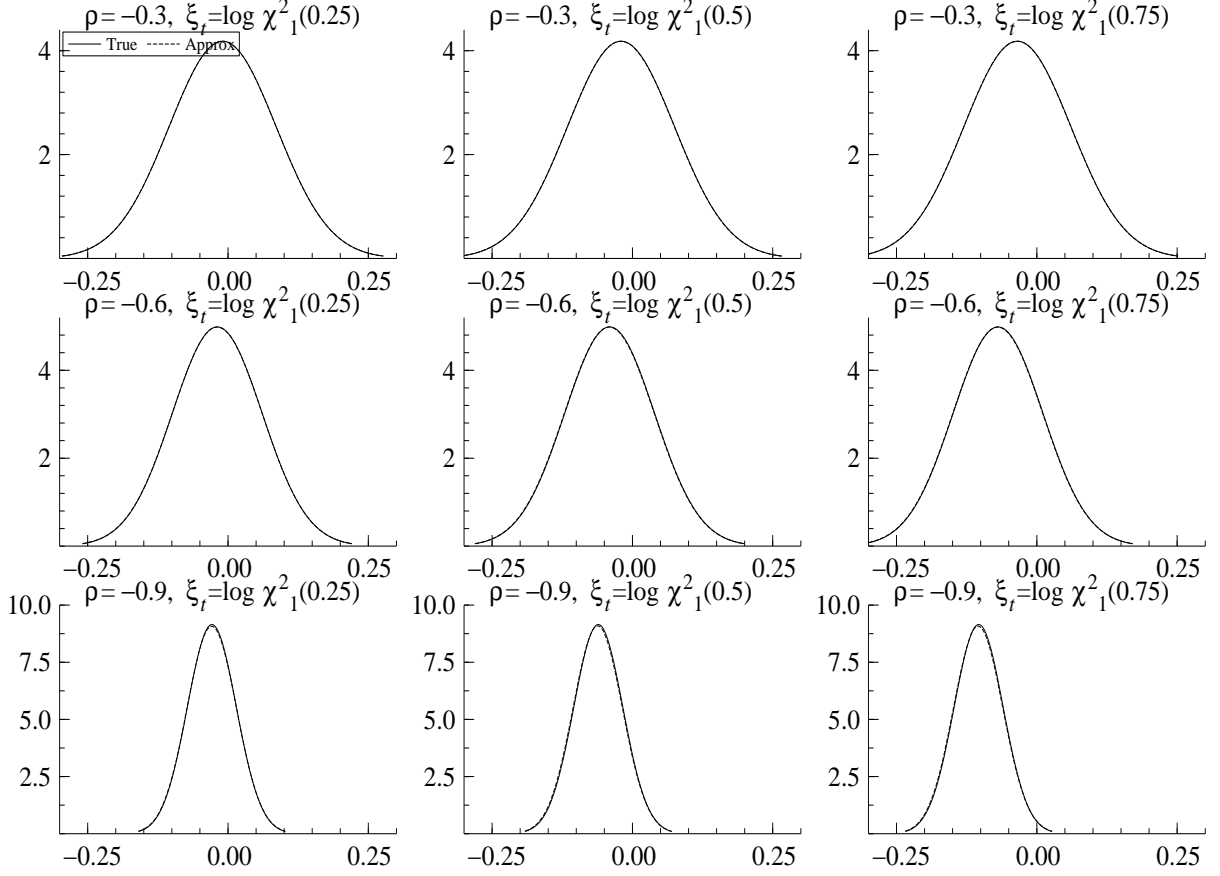
Figure 2: The conditional density of \eta_t given d_t = 1 and \xi_t = \log \chi_1^2(0.25) , \log \chi_1^2(0.5) , \log \chi_1^2(0.75) (left, middle, right) for \rho = -0.3, -0.6, -0.9 (top, middle, bottom).
