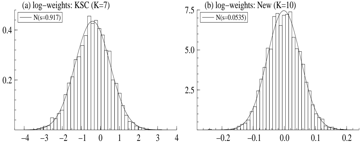
Figure 6: Histogram of the \log(w^{(i)} \times M) where M = 5,000 is a number of samples for a symmetric stochastic volatility model ( \rho = 0 ). Left: KSC ( K = 7 ). Right: New ( K = 10 ). Other line: the normal density function setting its mean and variance equal to the sample mean and sample variance.
