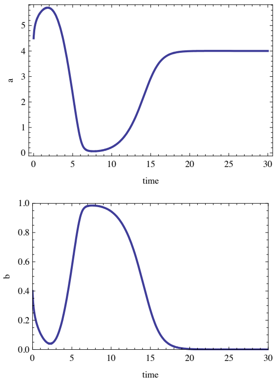
Figure 15: Mean dynamics in NK Model with a 4% target and optimal policy without commitment.
