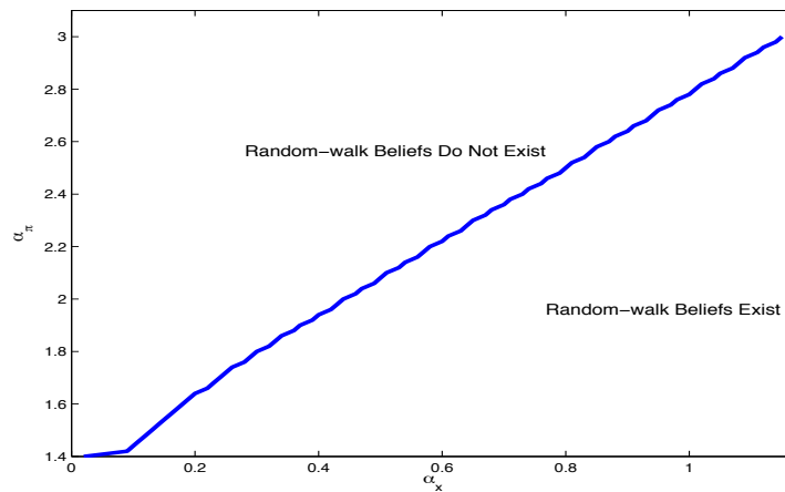
Figure 11: A Policy Frontier for Random-walk beliefs. All pairs of policy coefficients (\alpha_x, \alpha_\pi) below the line can lead to random-walk beliefs in the mean dynamics for the NK model with the baseline calibration, and policy coefficients above the line do not exhibit random-walk beliefs.
