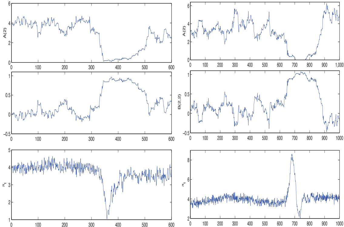
Figure 10: Inflation dynamics in NK Model with a 4% target.
