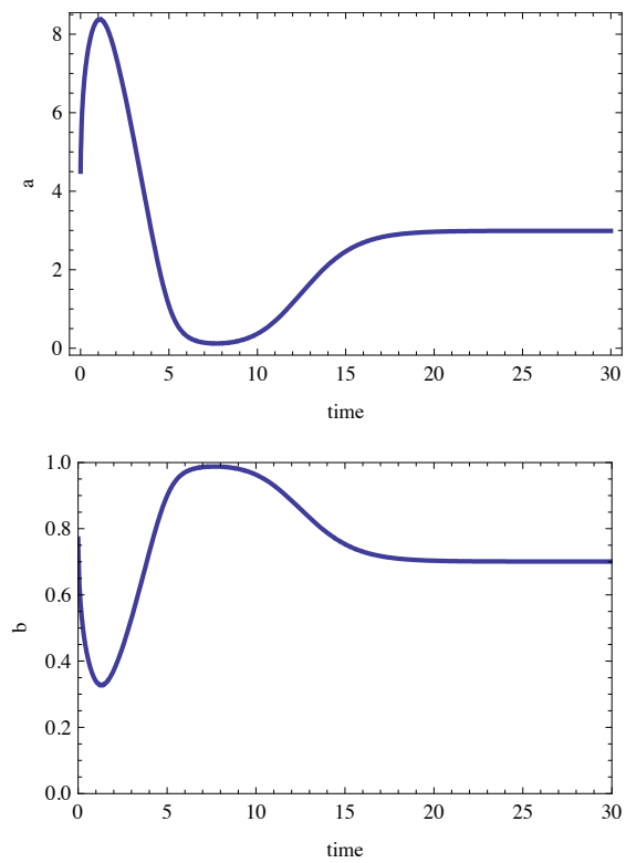
Figure 16: Mean dynamics in NK Model with a price-level targeting rule.
